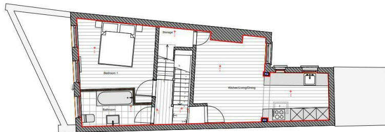
First Floor Plan Scale 1:100 @ A3
